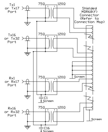
Balun Circuit For Each MDR68 (68 Way SCSI)
